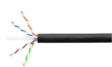
GigaSPEED X10D® 1091B ETL Verified Category 6A U/UTP Cable, black jacket, 4 pair count, 1000 ft (305 m) length, reel
