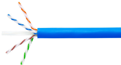
GigaSPEED X10D® 1091B ETL Verified Category 6A U/UTP Cable, blue jacket, 4 pair count, 1000 ft (305 m) length, reel
