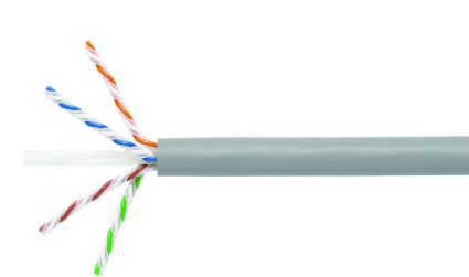
GigaSPEED X10D® 1091B ETL Verified Category 6A U/UTP Cable, slate jacket, 4 pair count, 3000 ft (914 m) length, reel
