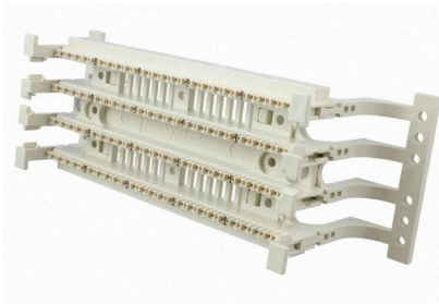
110Connect XC System Copper Wiring Block Kit, UTP term., 100-pair, 5-pair connecting blocks
