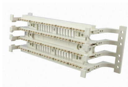
110Connect XC System Cross-Connect Wiring Block with Legs, 100-pair, Category 5e, .110 punch down
