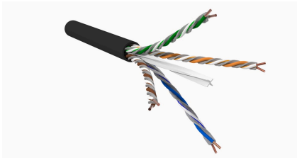
GigaREACH™ XL "Extended Distance" 1573A Category 6 U/UTP Cable, gel-filled outdoor, black jacket, 4 pair count, 3000 ft (915 m) length, reel
