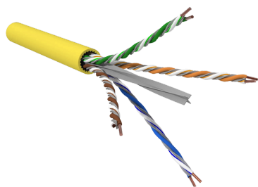
GigaREACH™ XL 2073A Category 6 U/UTP Cable, CMP Plenum, yellow jacket, 4 pair count, 1000 ft (305 m) length, reel
