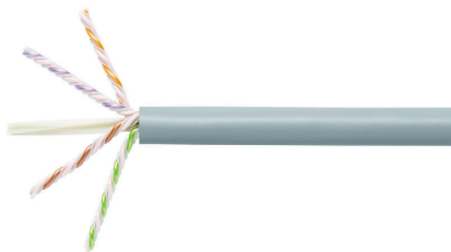
GigaSPEED X10D® 2091B ETL Verified Category 6A U/UTP Cable, slate jacket, 4 pair count, 1000 ft (305 m) length, reel
