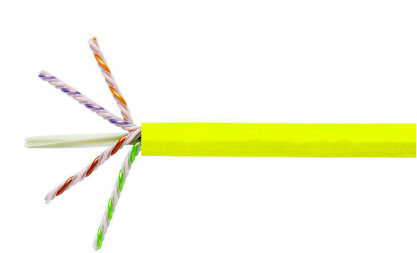
GigaSPEED X10D® 2091B ETL Verified Category 6A U/UTP Cable, yellow jacket, 4 pair count, 1000 ft (305 m) length, reel
