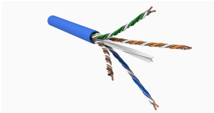
GigaREACH™ XL 3073A Category 6 U/UTP Cable, low smoke zero halogen, blue jacket, 4 pair count, 1640 ft (500 m) length, reel
