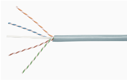
GigaSPEED X10D® 3091B ETL Verified Category 6A U/UTP Cable, slate jacket, 4 pair count, 1000 ft (305 m) length, WE TOTE® box
