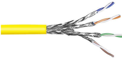
3297B Category 7 S/FTP Cable, low smoke zero halogen, yellow jacket, 4 pair count, 1640 ft (500 m) length, reel
