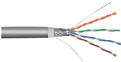
Copper Cable, category 5e, 4 pair, SF/UTP, CM, 24 AWG solid, 1000 ft, gray
