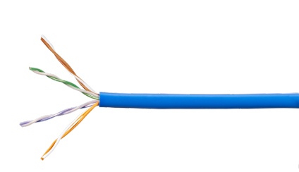
Copper Cable, category 5e, 4 pair, U/UTP, CM rated, 24 AWG, 1000 ft, blue
