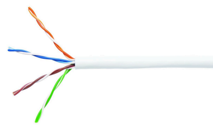
Copper Cable, category 5e, 4 pair, U/UTP, CM rated, 24 AWG, 1000 ft, white
