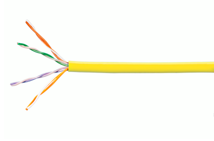
Copper Cable, category 5e, 4 pair, UTP, CM rated, 24 AWG, 1000 ft, yellow
