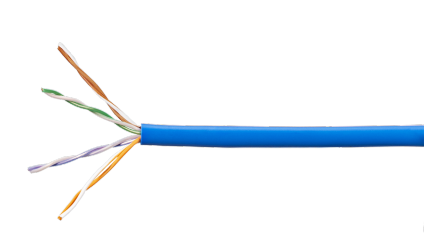
Copper Cable, category 5e, 4 pair, UTP, 350 MHz, CMR rated, 1000 ft pull-box, blue
