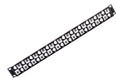
iPatch® M4200i 24 Port UTP Intelligent Universal Modular Panel without Modules
