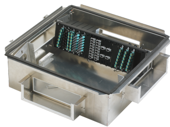
Raised Floor Enclosure, Wide Flange, 24"W x 24"L x 7"D with mount for management bracket
