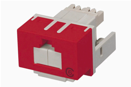
SX-Series Modular Jack, RJ45, Cat6 Unshielded, with Shutter, Red
